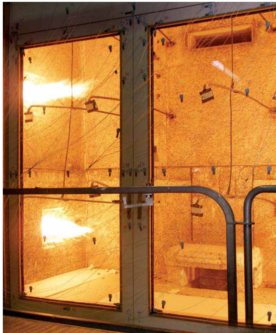
Testing of fire behaviour in accordance with DIN EN 1634-1.
