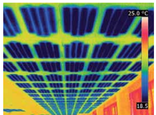
Thermal imaging to verify the performance of the chilled ceilings.
