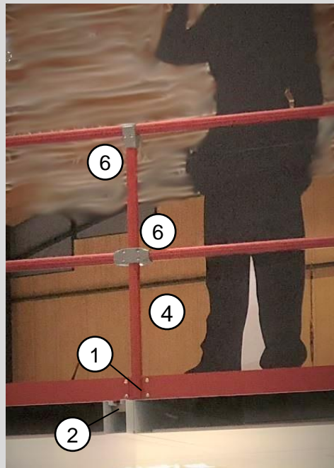
Image 2 Single parts of fall protection device
